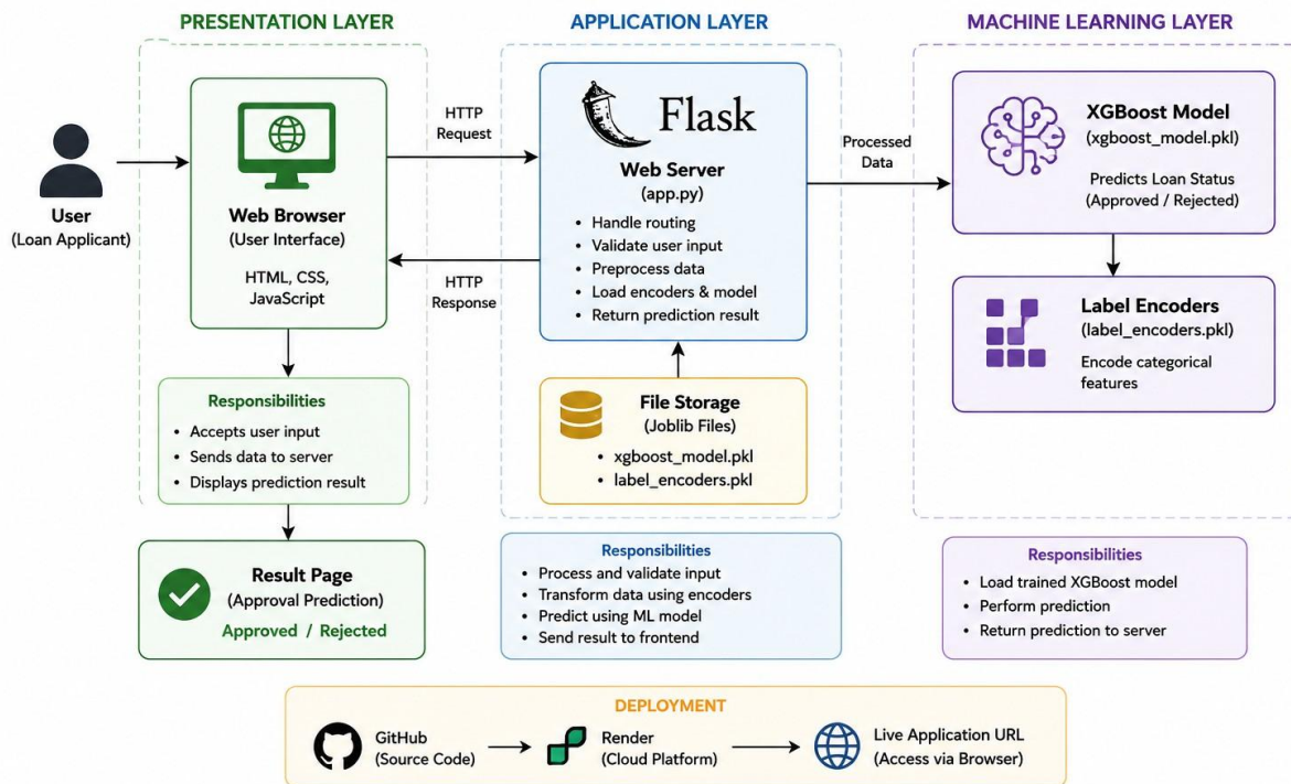
Technical Architecture Diagram
